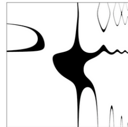
dłutoma (x^2 \cos(3x^2) + y^2 \cos(3y^2))^2 < 0.001
